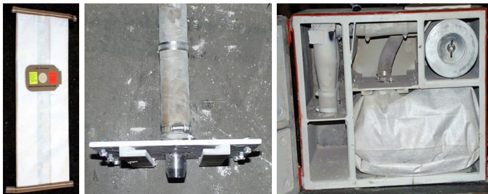
Figure 4.22. Dust collector bag (left), bag nozzle (center), and bag positioned in collector box and filled with dust (right).
